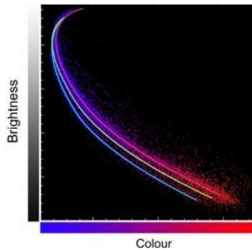
Each point in this graph represents one star in NGC 2808. The vertical axis represents each star's brightness, with the brightest stars near the top. The horizontal axis represents the stars' colors, with bluer stars to the left and redder to the right. The three lines represent the three different stellar generations present in the globular cluster. M. Kornmesser and L. L. Christensen (ESA/Hubble) [larger image]
